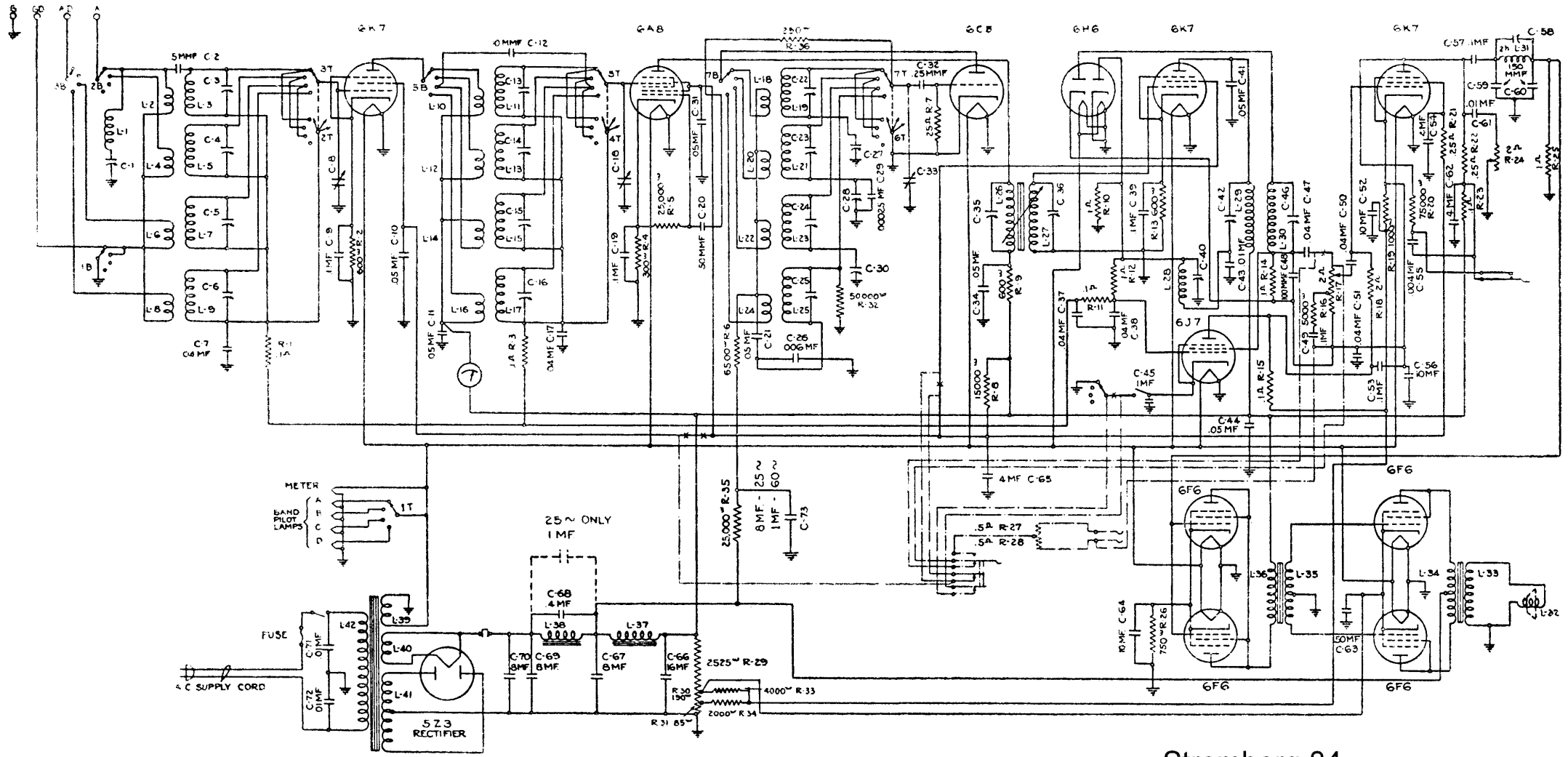
Fig. 2. Schematic Circuit of Receiver.
